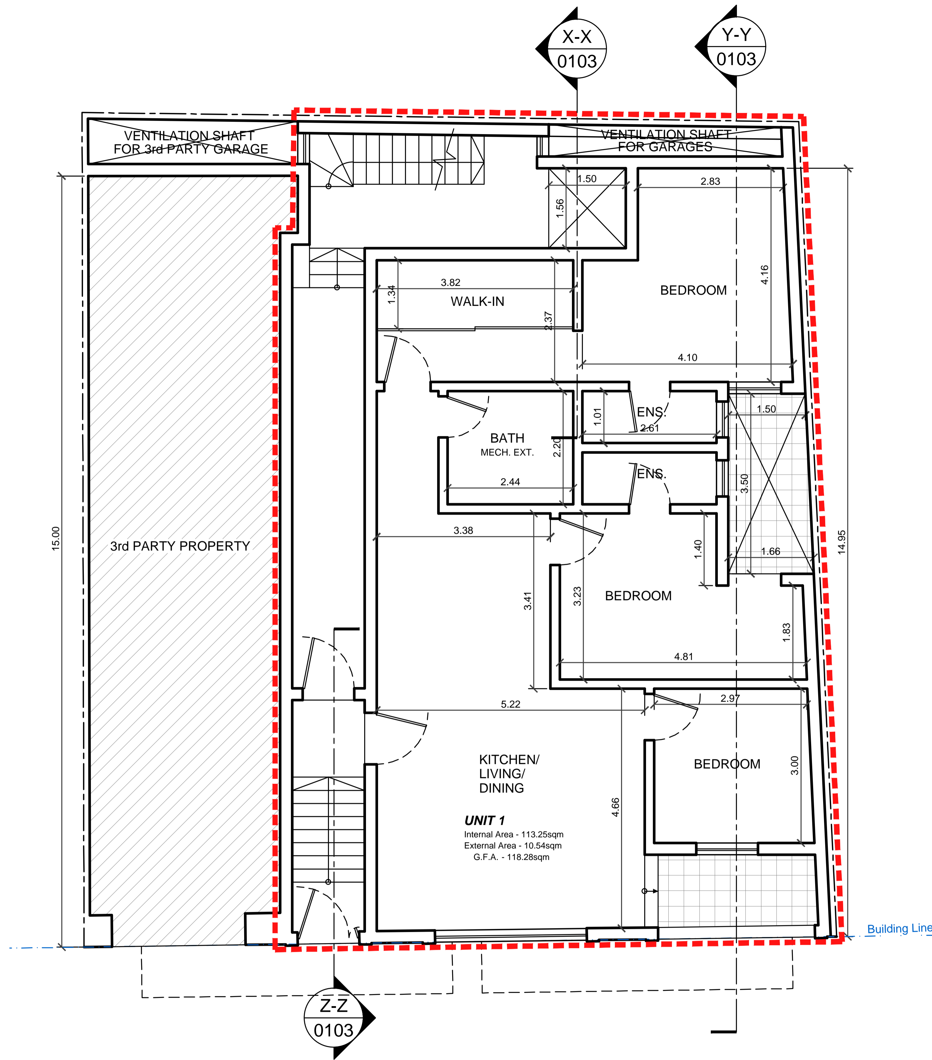
2 Proposed Ground Floor Level 1:100
